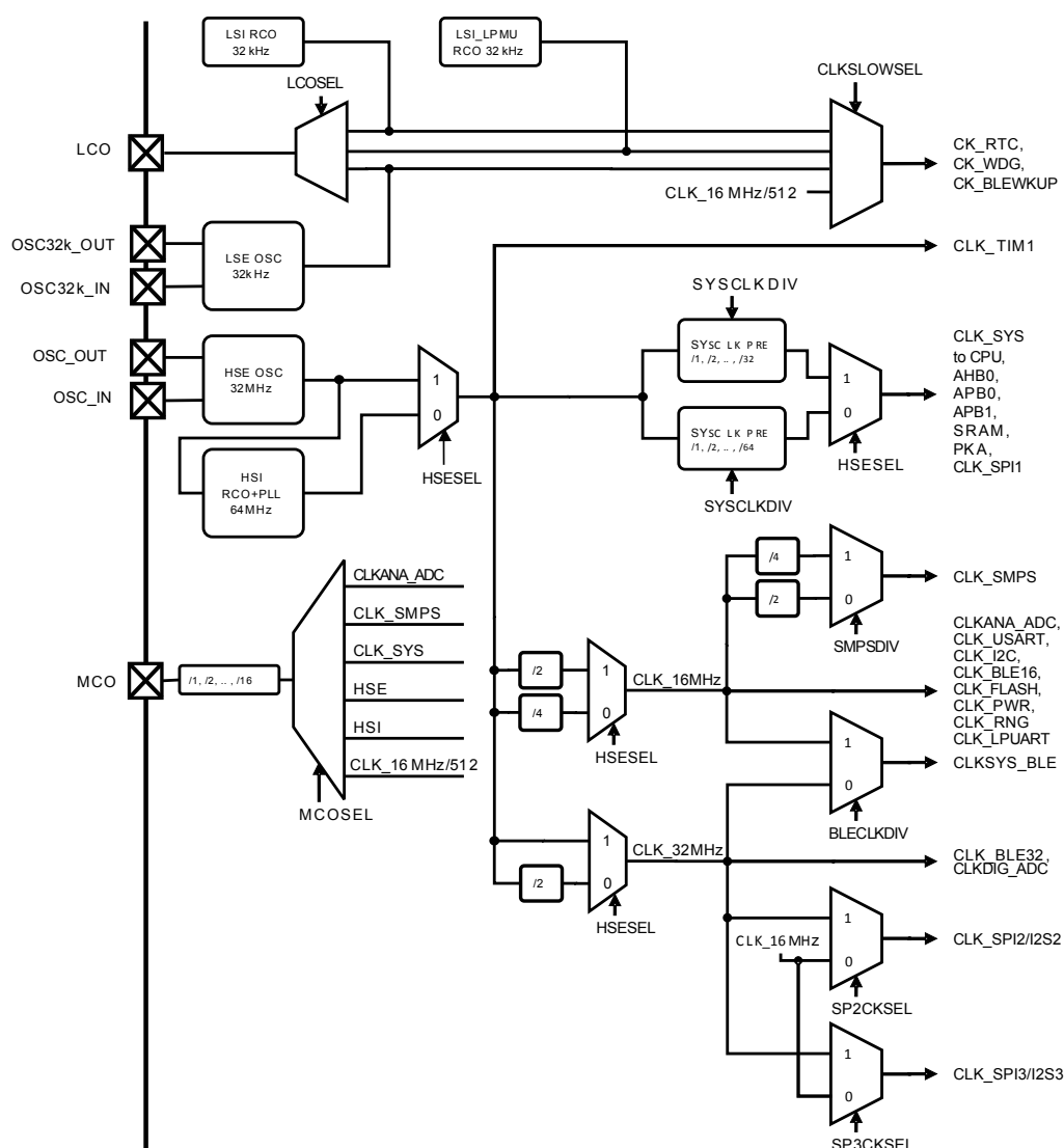
Figure 6. Clock tree
