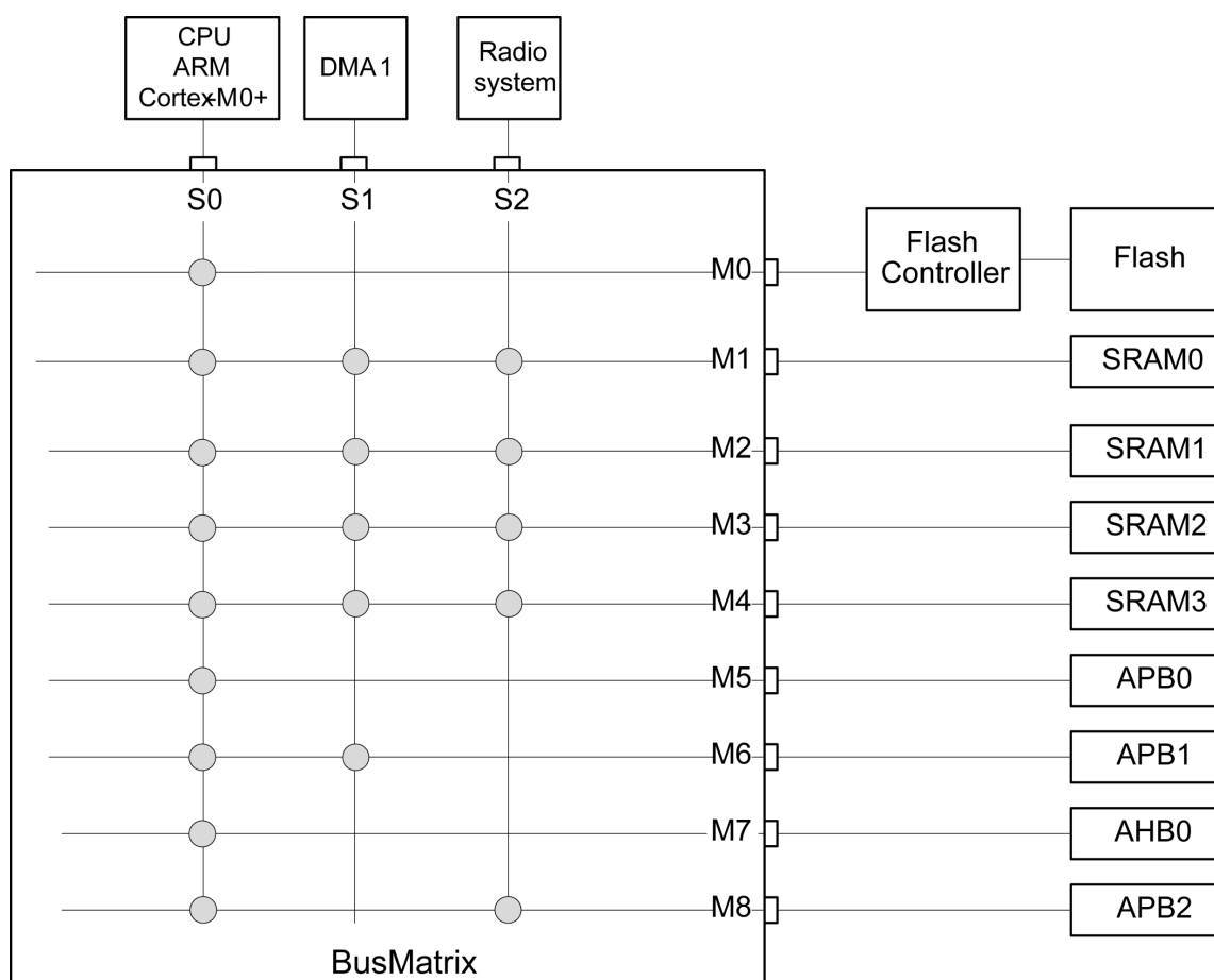
Figure 2. Bus matrix
