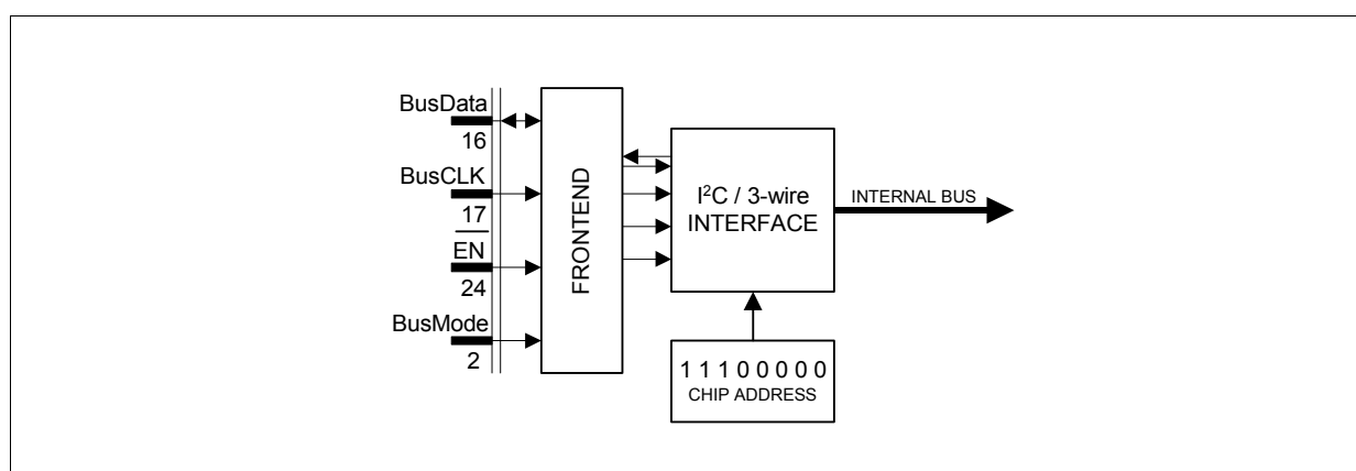
Figure 2-7 Bus Interface
