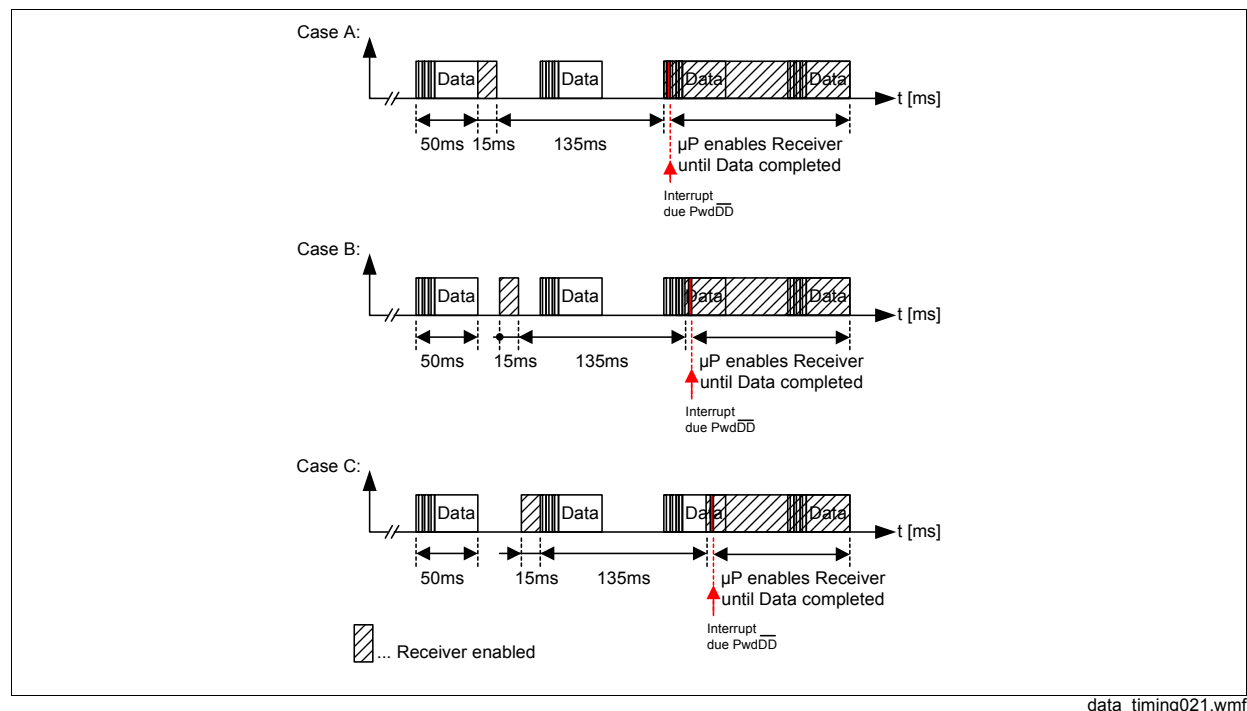
Figure 3-33 3 possible timings
