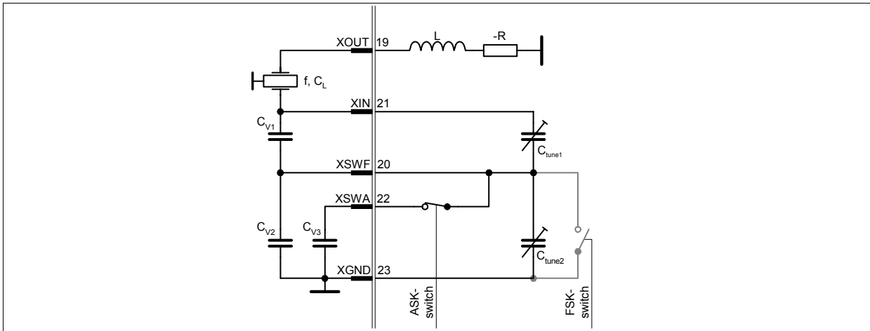
Figure 3-16 FSK receive
