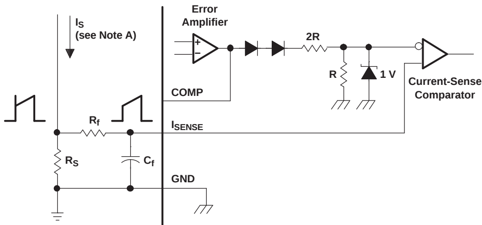
Figure 2. Current-Sense Circuit
