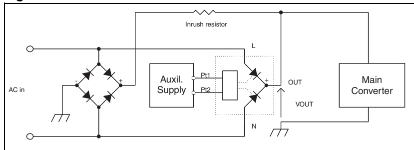
Figure 2: Basic connection
