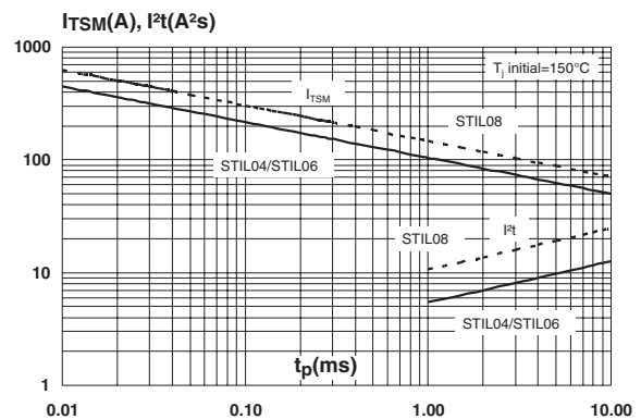
Figure 10: Non repetitive surge peak on-state current (sinusoidal pulse) and corresponding value of I^2t ( T_j initial = 150°C)
