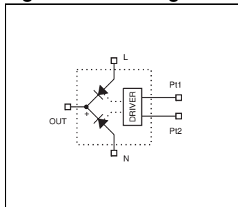
Figure 1: Block diagram
