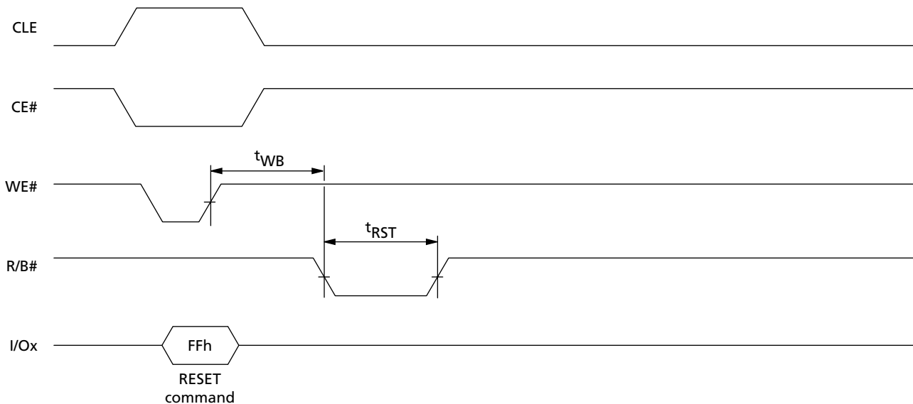
Figure 75: RESET Operation
