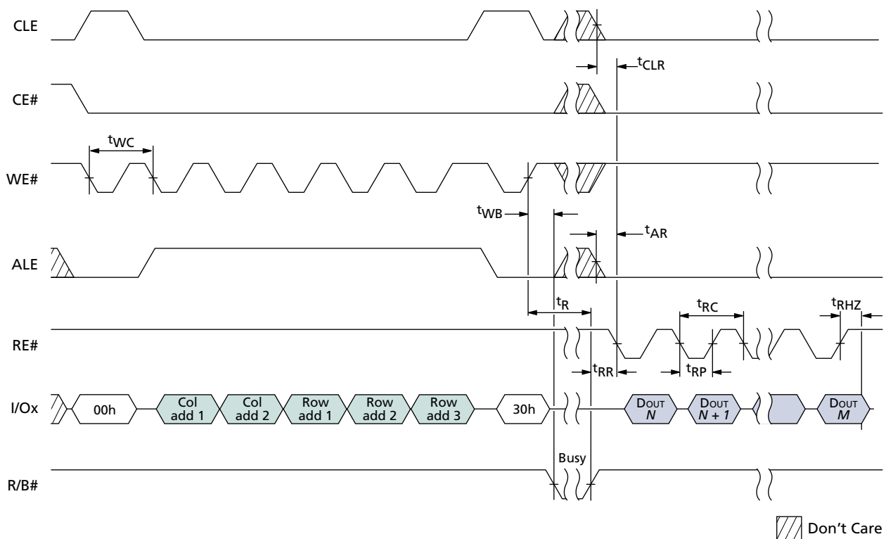
Figure 60: PAGE READ Operation
