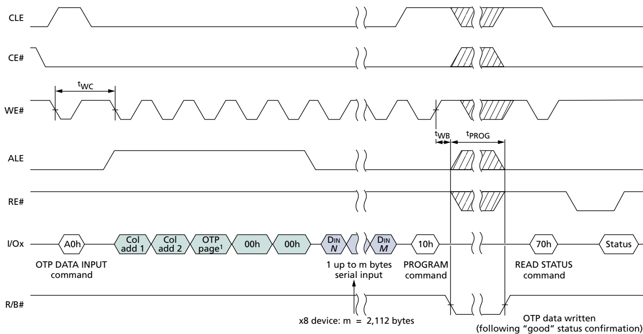
Figure 23: OTP DATA PROGRAM Operation
