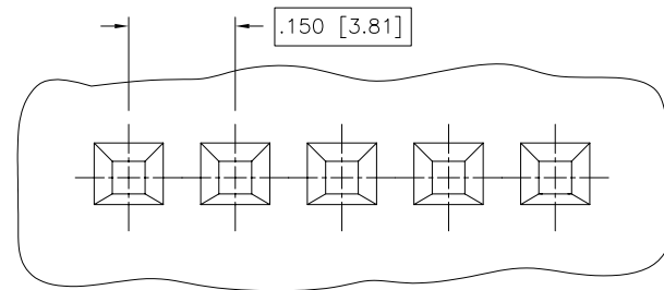
MATING PIN PATTERN SCALE 4/1
