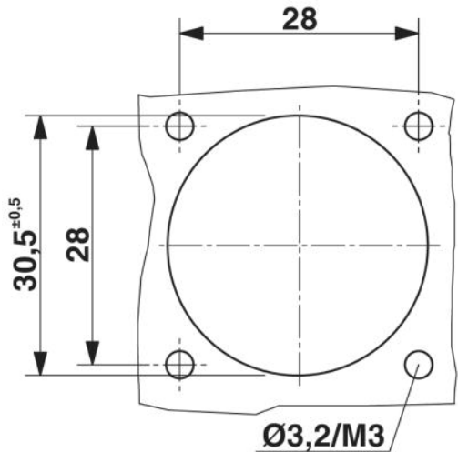
Panel cutout
