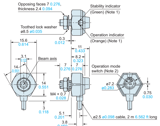
EX-33 EX-33-PN
