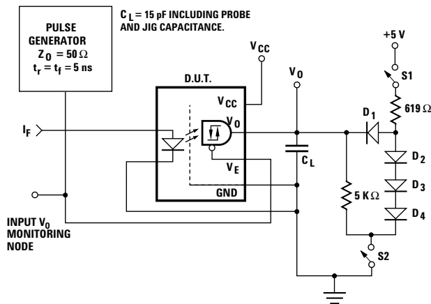
Figure 8. Test Circuit for t_{PHZ} , t_{PZH} , t_{PLZ} , and t_{PL} .
