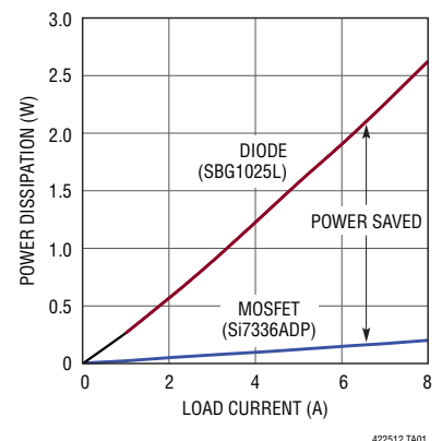
Power Dissipation vs Load Current
