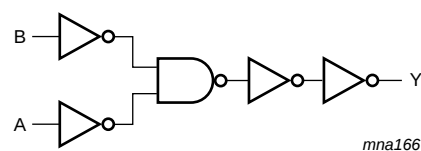
Fig 3. Logic diagram
