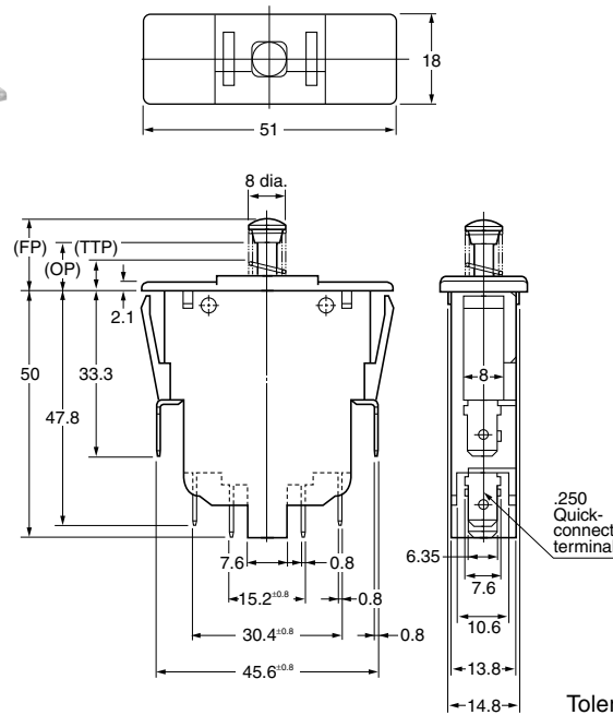
3 Form A type without button guard
