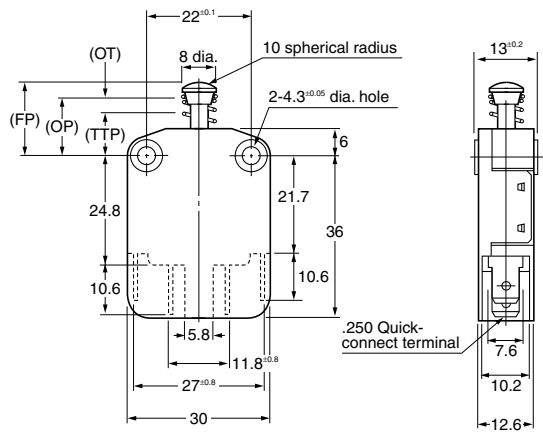
External dimensions
