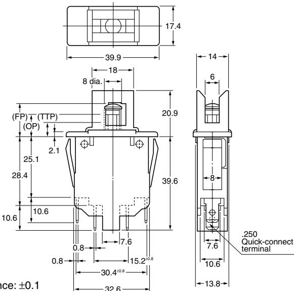
2 Form A type with button guard
