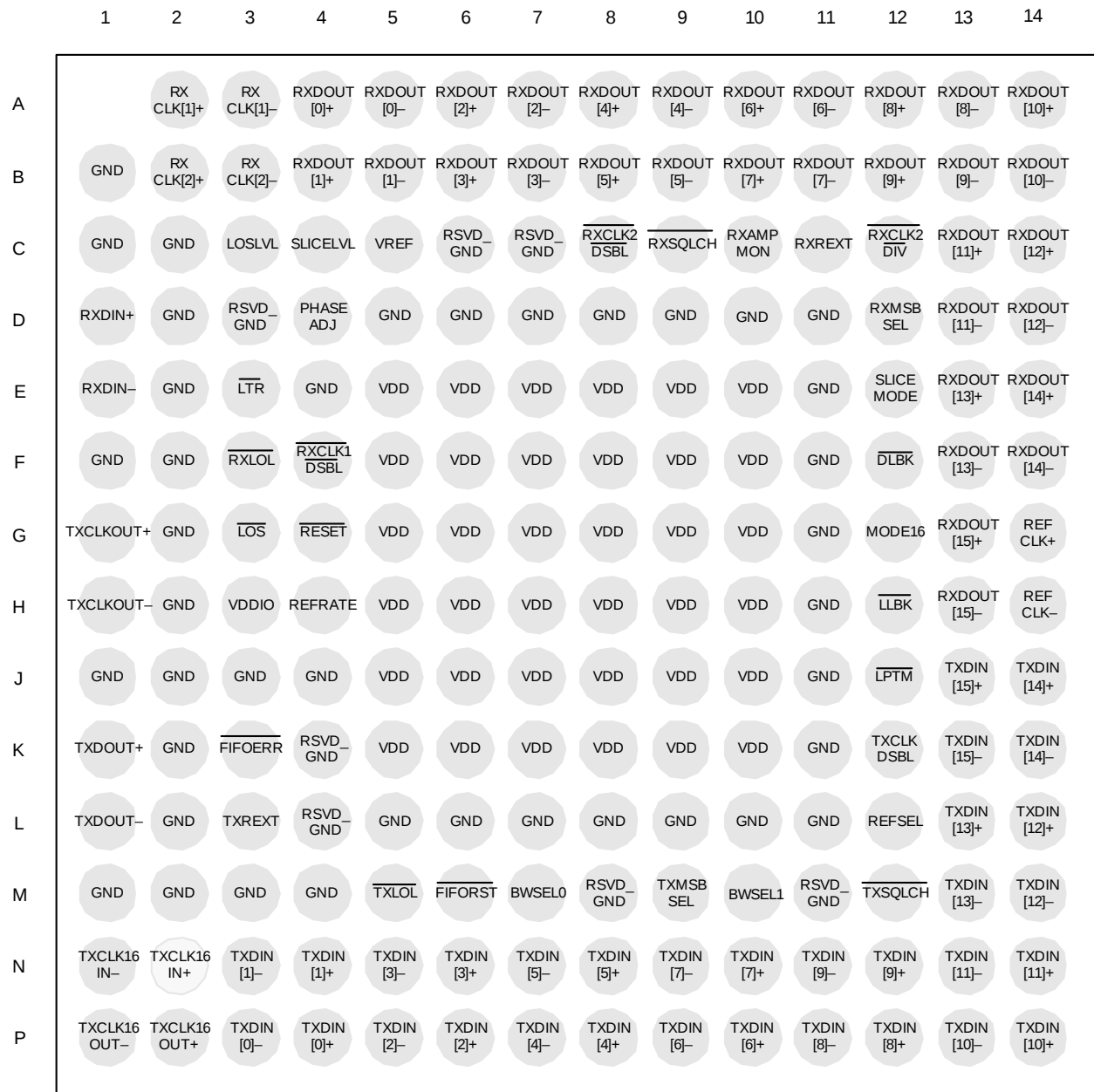
Figure 14. Si5100 Pin Configuration (Transparent Top View)
