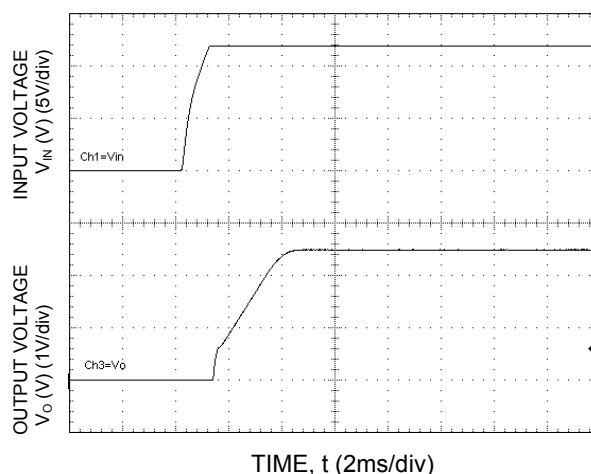
Fig-32. Typical Start-up Using Input Voltage (V IN = 12V, I o = I o,max ).
