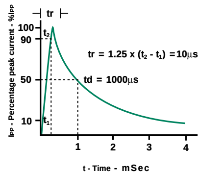
PULSE WAVE FORM (10/10000 \mu S)
