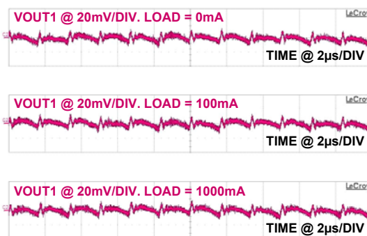
FIGURE 23. PWM1 OUTPUT RIPPLE, MODE = 5V (CCM)
