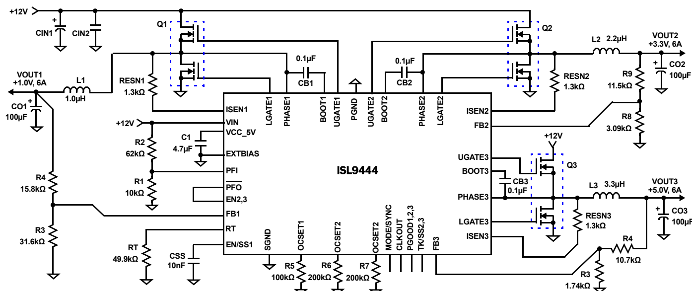
FIGURE 1. TYPICAL APPLICATION
