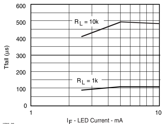
Fig. 8 t_{fall} vs. Forward Current
