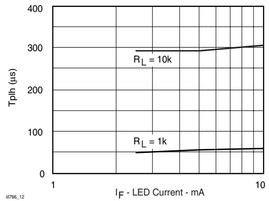
Fig. 12 t_{plh} vs. Forward Current
