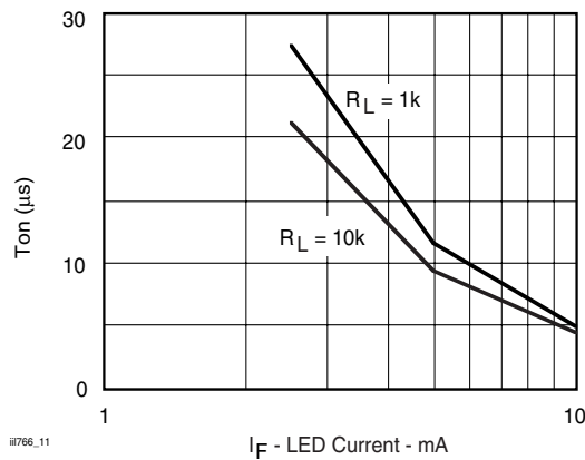
Fig. 11 t_{phl} vs. Forward Current
