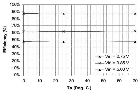
Typical Efficiency vs T_a I_{out} = 5 mA
