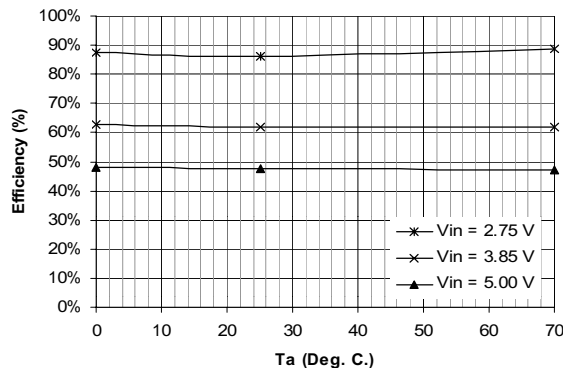
Typical Efficiency vs T_a I_{out} = 20 mA
