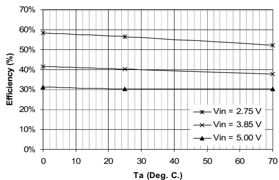
Typical Efficiency vs T_a I_{out} = 10 uA
