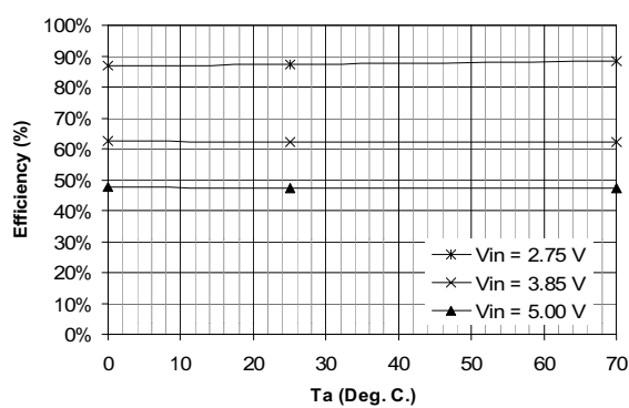
Typical Efficiency vs T_a I_{out} = 10 mA
