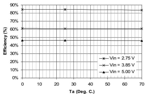
Typical Efficiency vs T_a I_{out} = 200 uA
