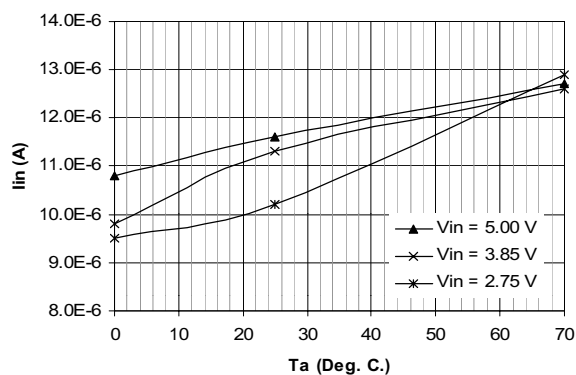
Typical I_{in} vs T_a I_{out} = 0
