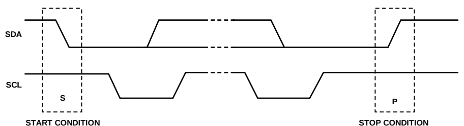
Figure 52. Start and Stop Conditions
