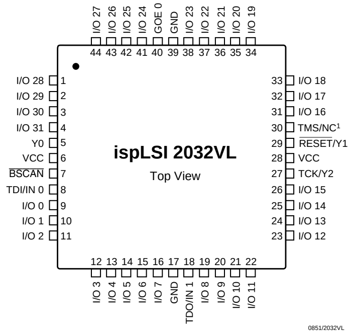
ispLSI 2032VL 44-Pin TQFP Pinout Diagram
