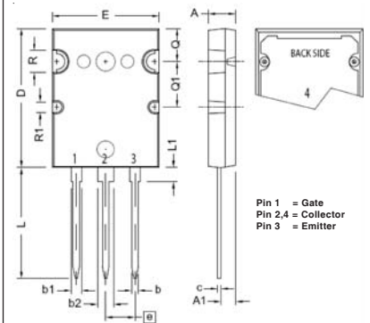
PLUS264™ (IXYB) Outline
