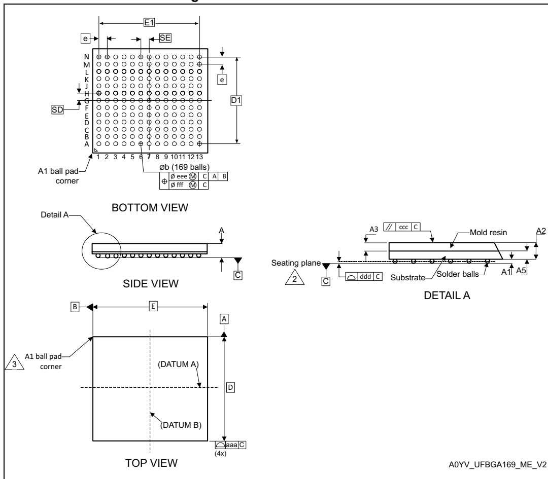
Figure 73. UFBGA169 - Outline
