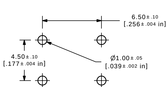
P.C. MOUNTING
