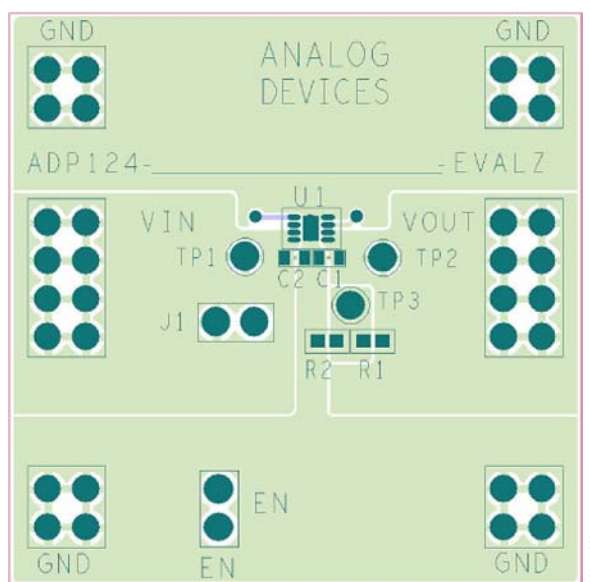
Figure 3. ADP124 MSOP Evaluation Board Layout
