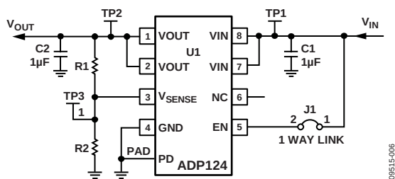
Figure 6. ADP124 Evaluation Board Schematic, LFCSP
