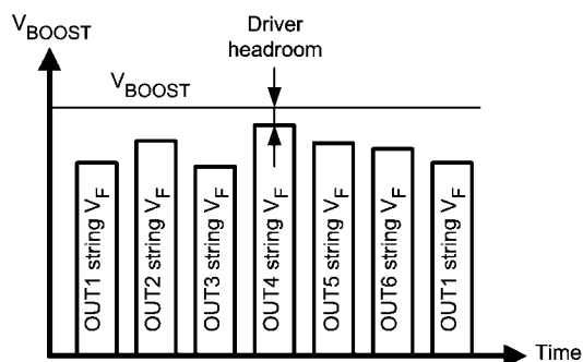
Boost Adaptive Control Principle with PSPWM
