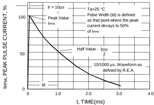
FIG.3 - PULSE WAVEFORM
