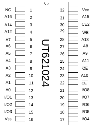
PDIP / SOP
