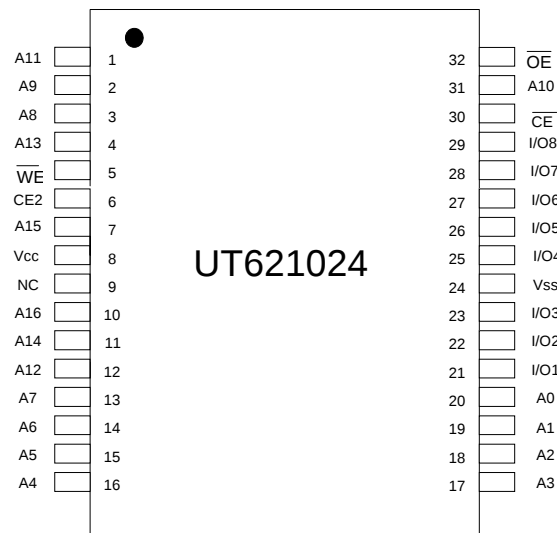
TSOP-I/STSOP
