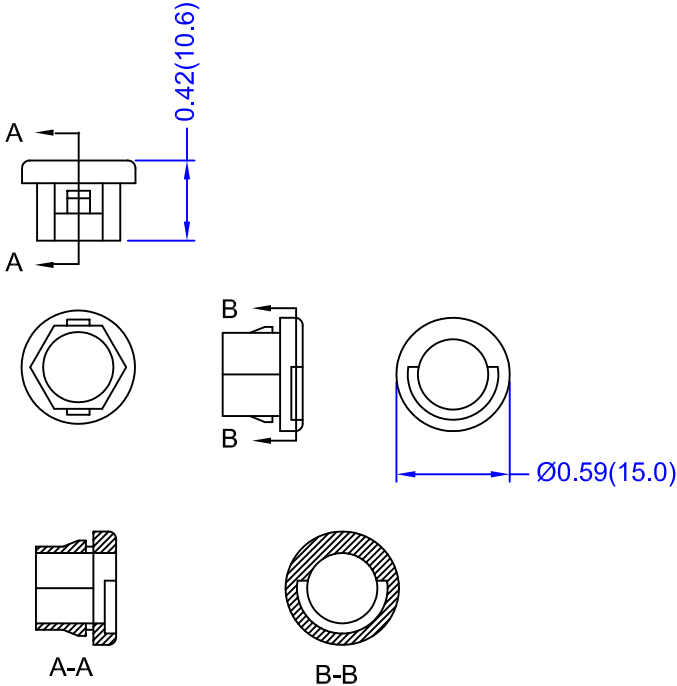
Clip Nut Details
