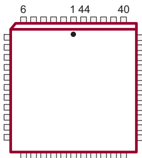
44-lead PLCC (Top view)
