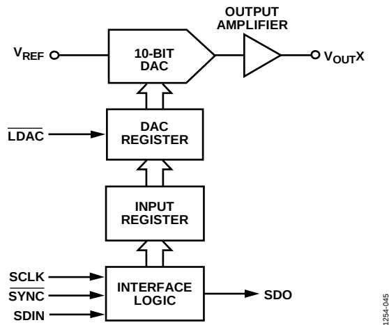
Figure 43. Simplified Diagram of Input Loading Circuitry for a Single DAC
