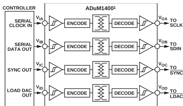
Figure 50. Isolated Interface
