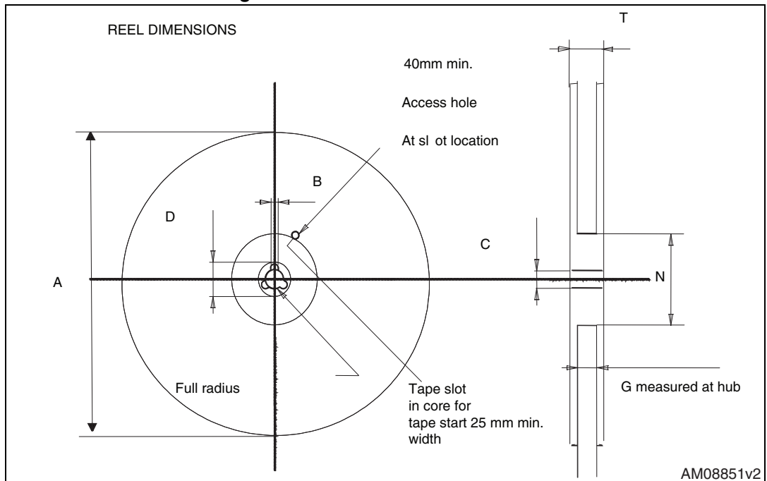
Figure 41. Reel for DPAK and D 2 PAK
