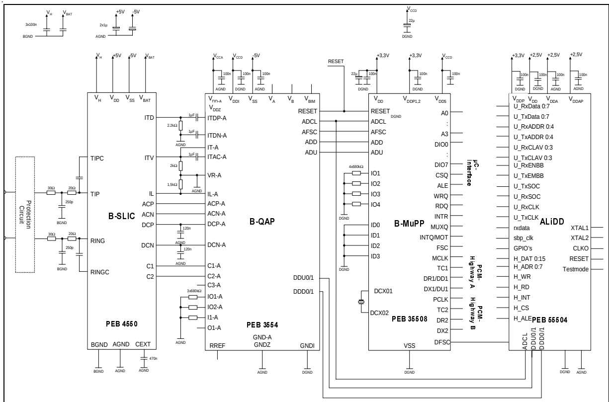
Figure 5-1 Application Circuit
