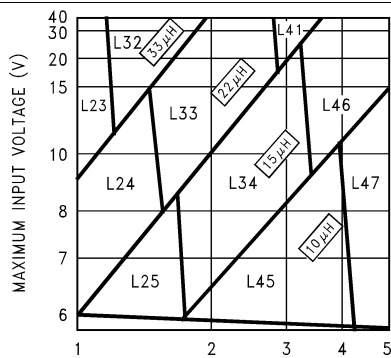
Figure 14. LM2679-3.3 V
