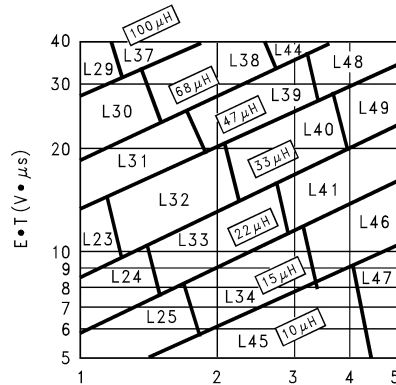
Figure 17. LM2679-Adjustable Voltage
