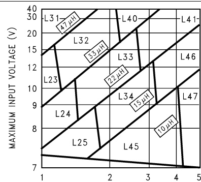
Figure 15. LM2679-5 V
