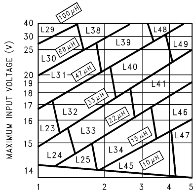
Figure 16. LM2679-12 V
