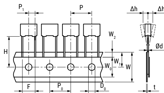
Figure 2 – Lead Spacing 7.5 mm
