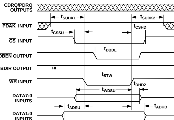
Figure 21. Control Register/PIO Write Cycle
