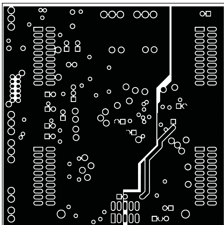
Figure 32. TLV320AIC3105EVM Layer 4
