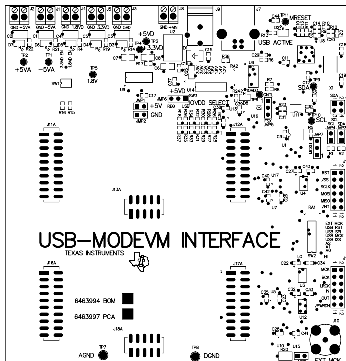
Figure 37. USB-MODEVM Assembly Layer
