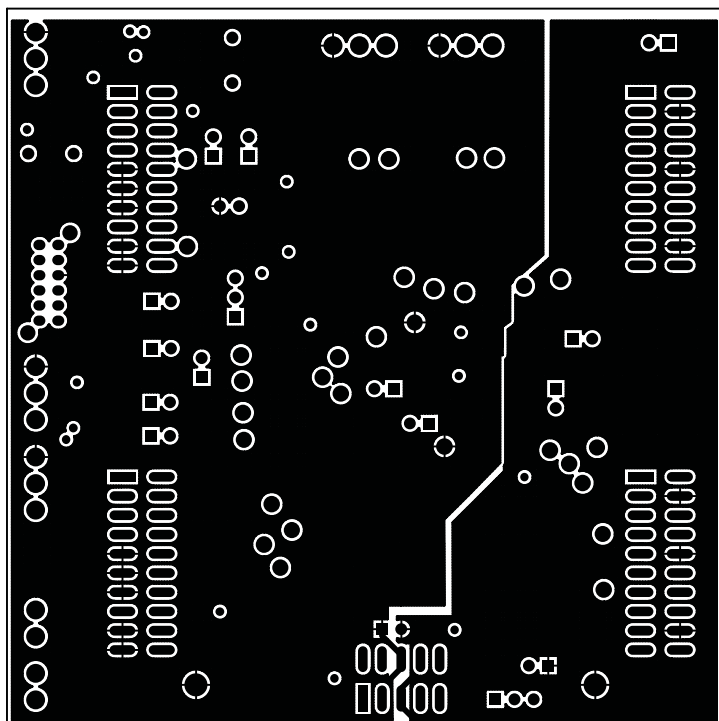
Figure 31. TLV320AIC3105EVM Layer 3
