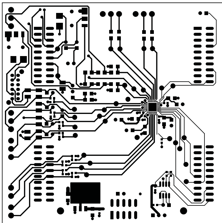
Figure 30. TLV320AIC3105EVM Top Layer
