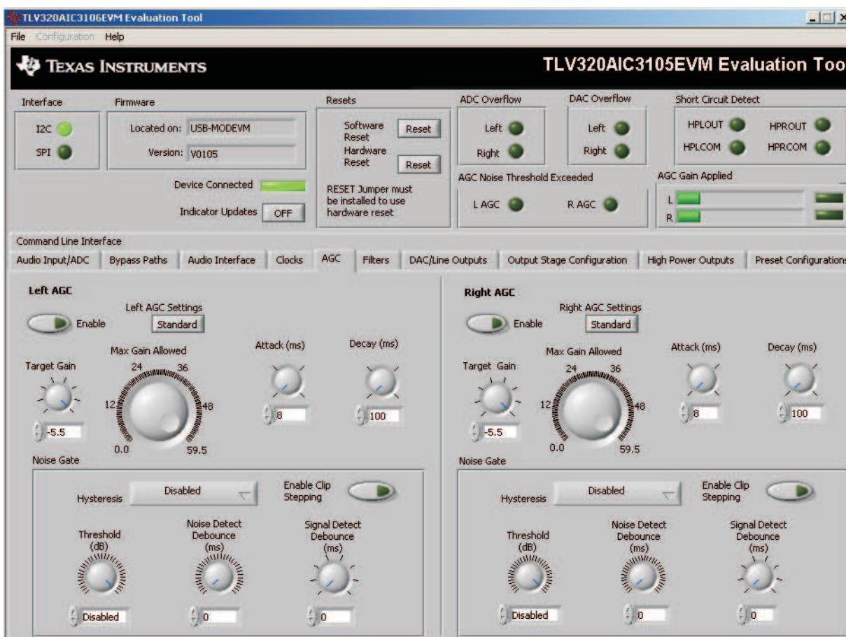
Figure 9. AGC Tab
