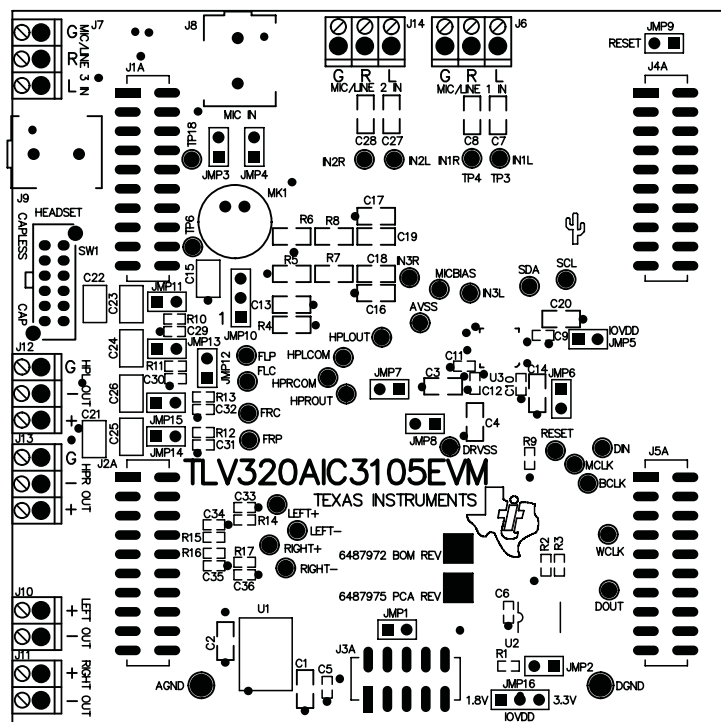
Figure 29. TLV320AIC3105EVM Assembly Layer
