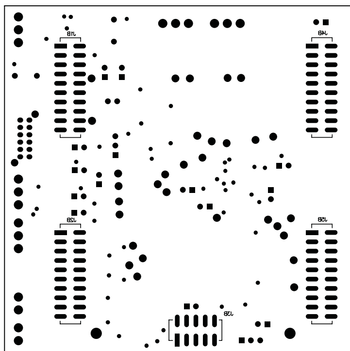
Figure 34. TLV320AIC3105EVM Bottom Layer
