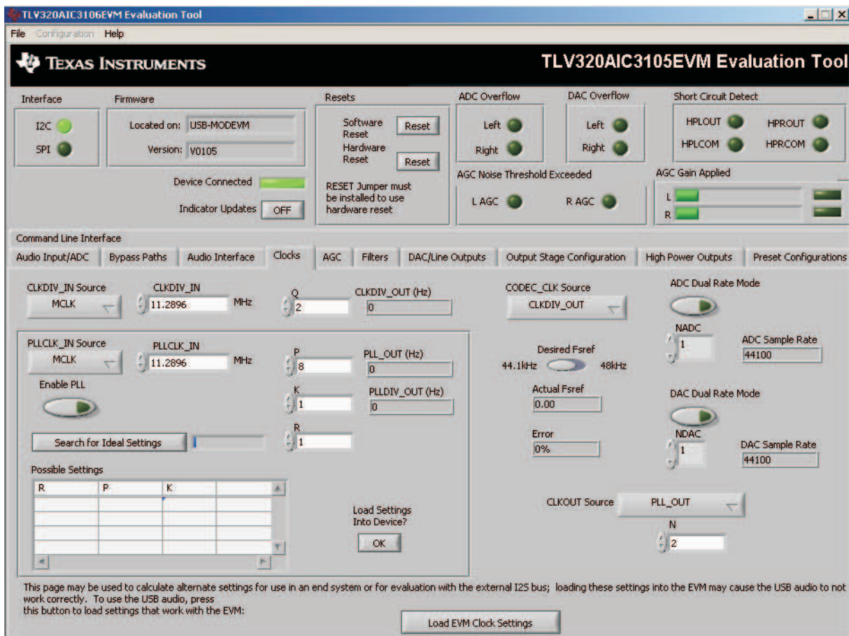
Figure 8. Clocks Tab
