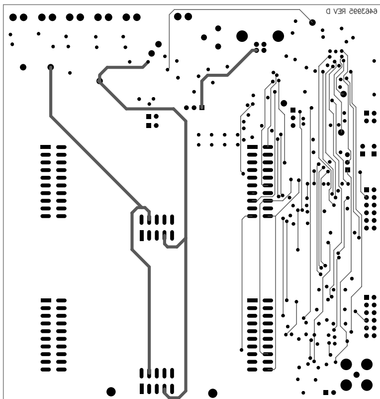
Figure 39. USB-MODEVM Bottom Layer
