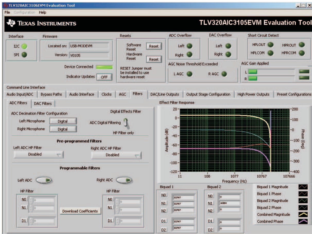
Figure 12. Filters Tab
