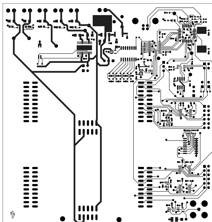
Figure 38. USB-MODEVM Top Layer
