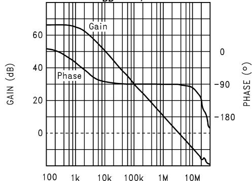
Open Loop Frequency Response V_{DD} = 3V , No Load
