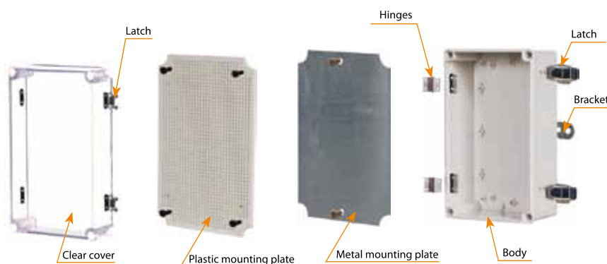
TIBOX 鎖扣安裝組裝圖 Pictures for mounting TIBOX Latch
