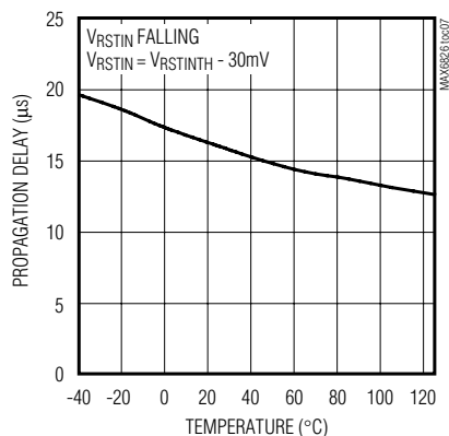
V RSTIN TO RESET OUTPUT DELAY vs. TEMPERATURE
