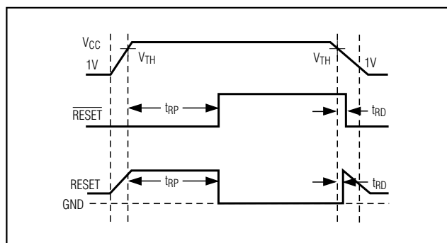
Figure 3. Reset Timing Diagram
