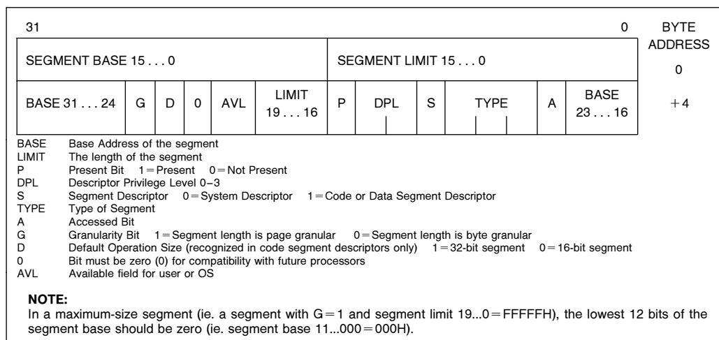
Figure 4-5. Segment Descriptors
