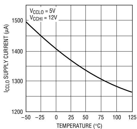
ICCL0 Supply Current vs Temperature
