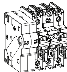
Left side rotary switch Counterclockwise operating handles
