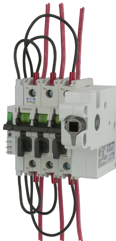
Right front rotary operated CCP2 switch with PLC fuse monitor.
