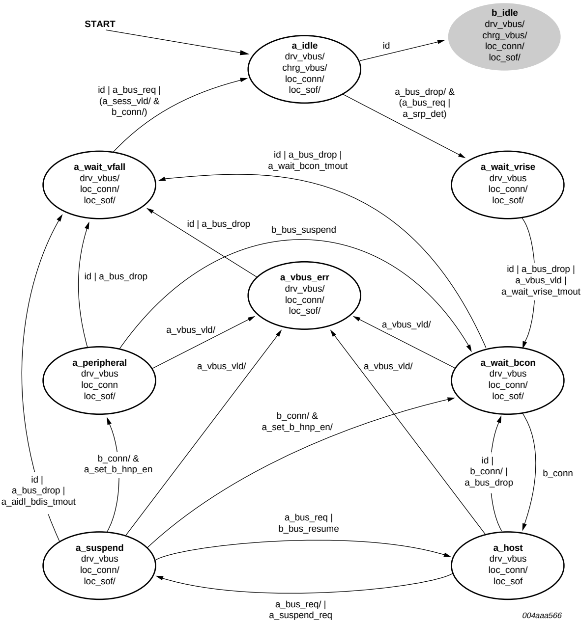
Fig 15. Dual-role A-device state diagram
