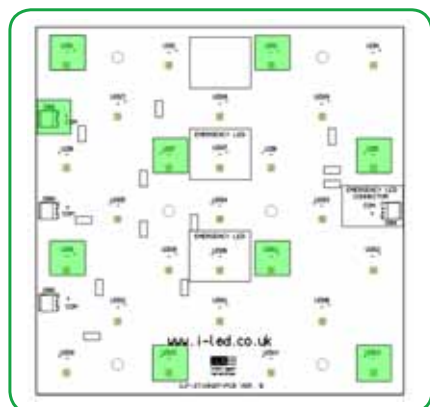
LEDs connected to CON4 - Emergency
