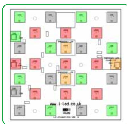
Connecting all main light LEDs together
