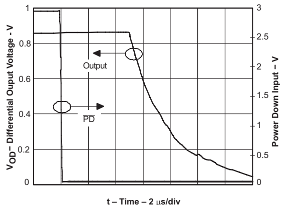
Figure 69. Turnoff Time
