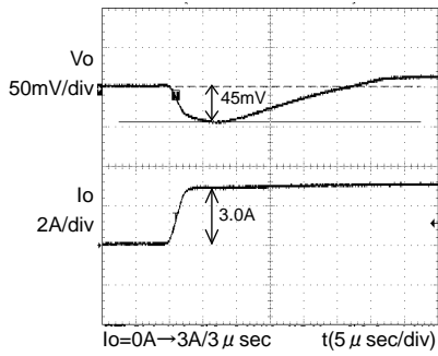
Fig.1 Transient response (0→3A) Co=150 \mu F \times 2
