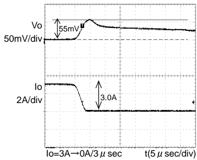
Fig.4 Transient response (3→0A) Co=150 \mu F \times 2
