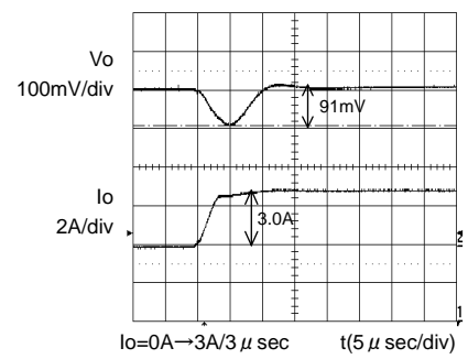
Fig.3 Transient response (0→3A) Co=47 \mu F
