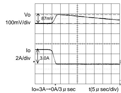
Fig.6 Transient response (3→0A) Co=47 \mu F
