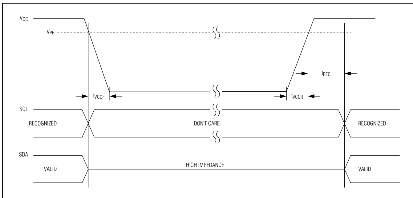
Figure 2. Power-Up/Power-Down Timing
