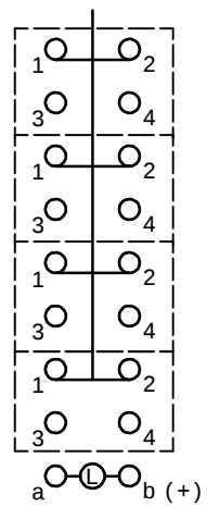
4PDT CONTACT CONFIGURATION
