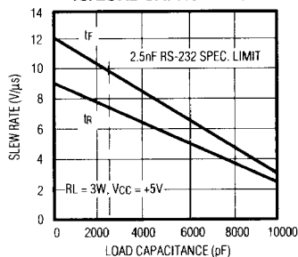
MAX252 TRANSMITTER SLEW RATE vs. LOAD CAPACITANCE
