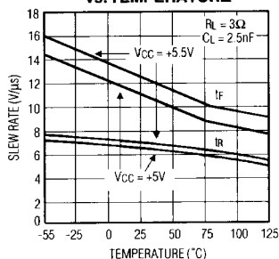
MAX252 TRANSMITTER SLEW RATE vs. TEMPERATURE
