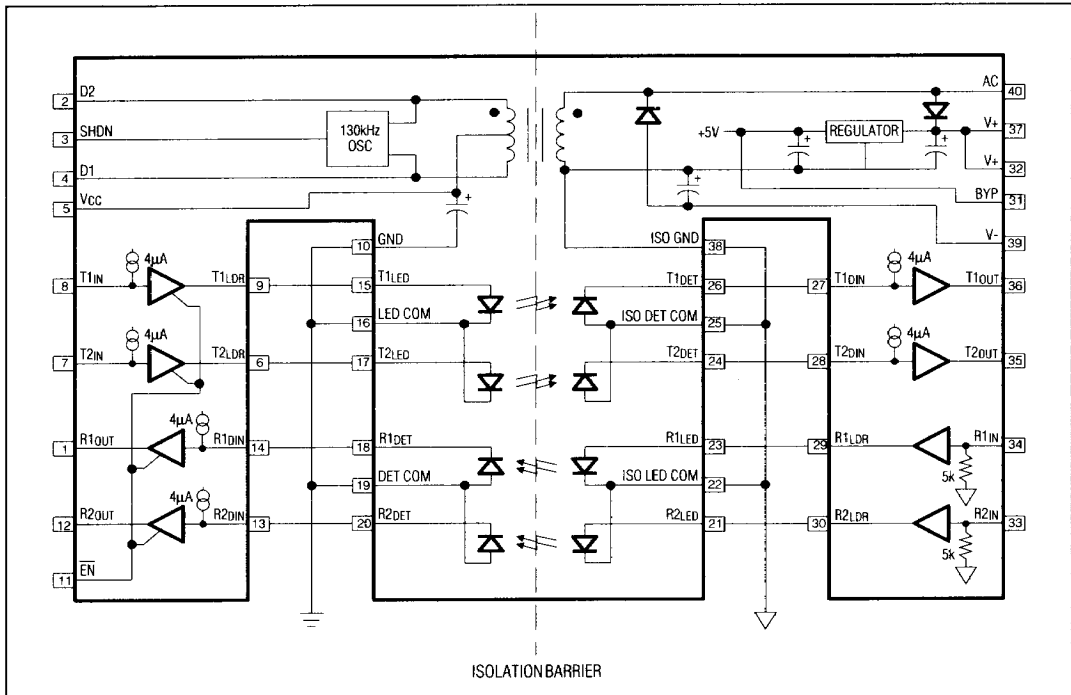
MAX252 Block Diagram
