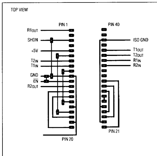
Figure 2. Preferred Layout
