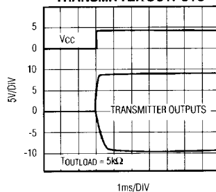
POWER-UP DELAY TO TRANSMITTER OUTPUTS
