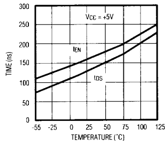
MAX252 ENABLE, DISABLE TIME vs. TEMPERATURE
