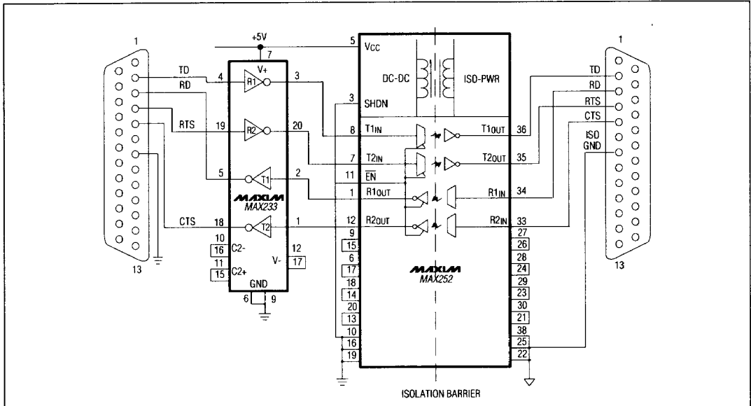
Figure 3. RS-232 Isolation Adapter from a Single +5V Supply
