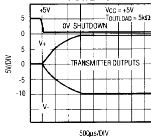
TIME FROM SHUTDOWN TO POWER-UP
