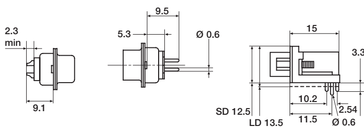
Solder Bucket
