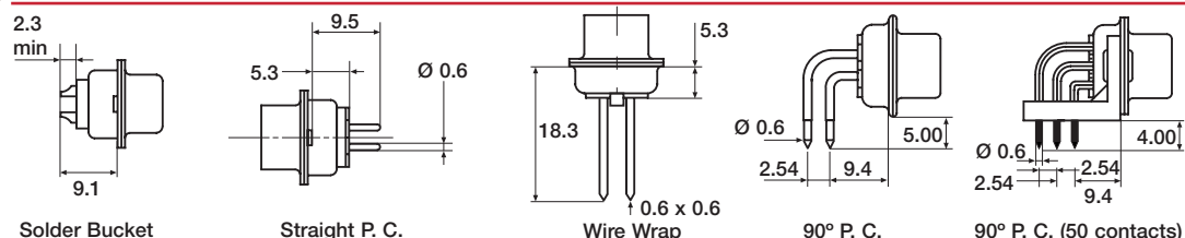
Solder Bucket
